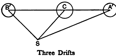
FIG. 16.—Comparison of Two-drift and Three-drift Theories.
